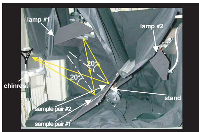
Figure 1. Side view of the booth built for gloss observations. Set up for illumination and observation at 20^\circ . Light path is highlighted in yellow. Lamp #2 is prepared for illumination and observation at 60^\circ , when the sample stand is in appropriate position. The two lamps and the stand are mounted on rotation and translation systems to allow an architecture of 5 and 4 deg of freedom, respectively. The booth is 1m x 1m x 1m. Black curtains allow the isolation of the booth from straylight. The light originates from two fluorescent tubes (15 W, 450-mm long) that illuminate several samples. The tubes have been set up according to the ASTM D4449-90 standard recommendations.
