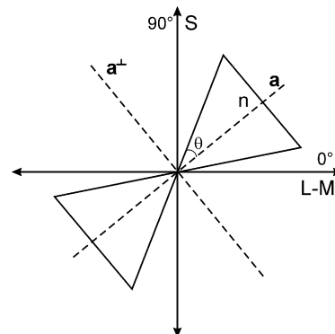
Fig. 1. Sectored noise of amplitude n that fills a sector in color space of half-width \theta , oriented along the direction \mathbf{a} .
