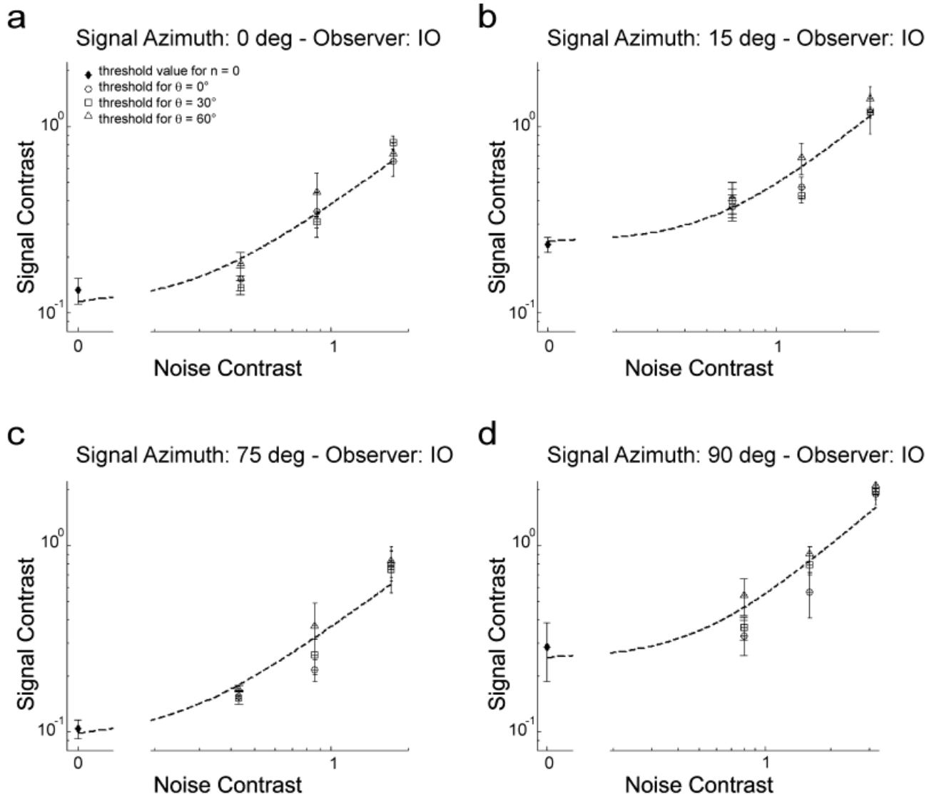
Fig. 2. Sectorised noise masking of a signal of azimuth 0 deg (a), 15 deg (b), 75 deg (c), and 90 deg (d). Noise-masking thresholds were measured for sector half-widths 0, 30, and 60 deg. Each data point represents the average of three staircases. Error bars represent the standard error of the mean. The dashed lines represent the best-fitting curves to s^2 = e_o + kn^2 . Results are for observer IO.
