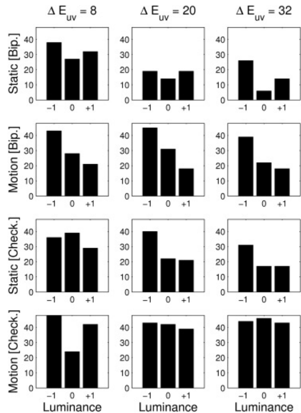
Fig. 4. Grouped results for translatory chromatic variations across the test overlay. Other details are as in Fig. 3.
