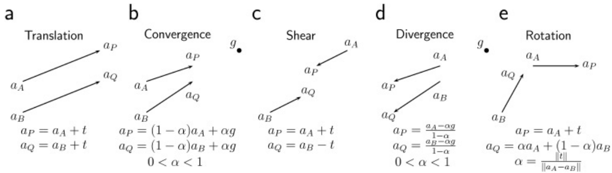
Fig. 2. Examples of each of the five chromatic variations used to define the color change in the test overlay. The tails of each vector, a_A and a_B , correspond to tristimulus coordinates outside the overlay, and the heads, a_P and a_Q , within. The equations define the rules relating interior to exterior tristimulus coordinates. In the above examples, t is a constant vector.
